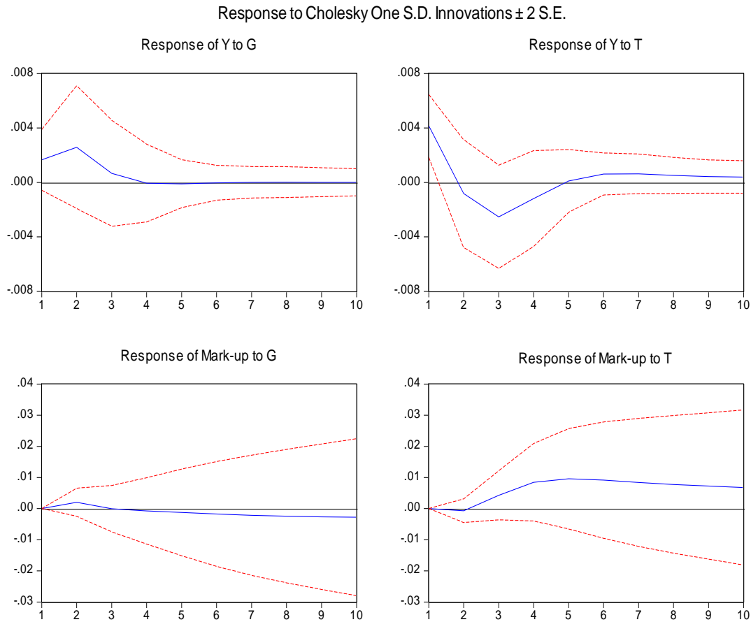
Figure 3: The impulse response functions
