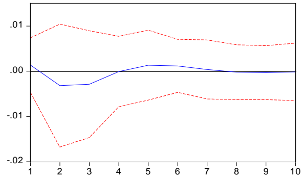
Response of Mark-up to T
