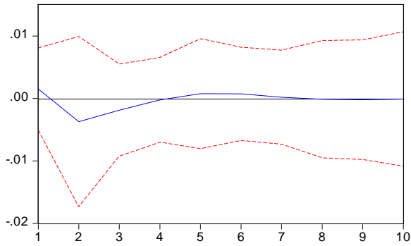
Response of Mark-up to G
