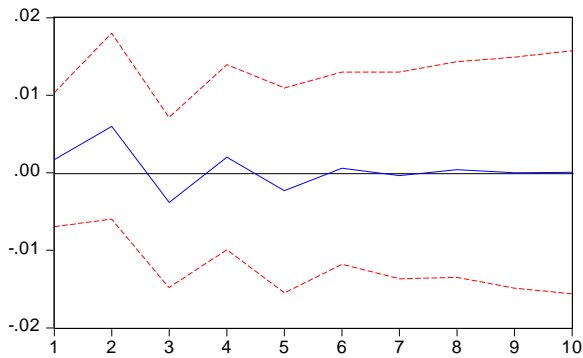
Response of Mark-up to G
