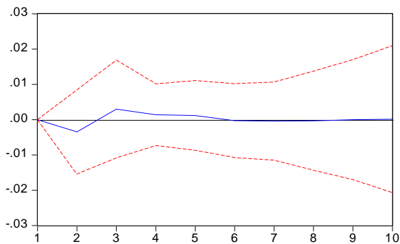
Response of PTF to G
