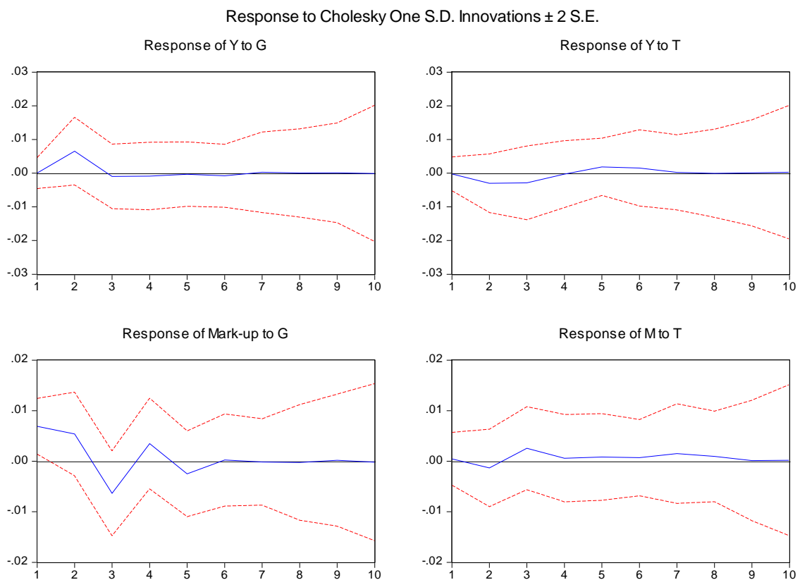
Figure 1: The impulse response functions: Italy
