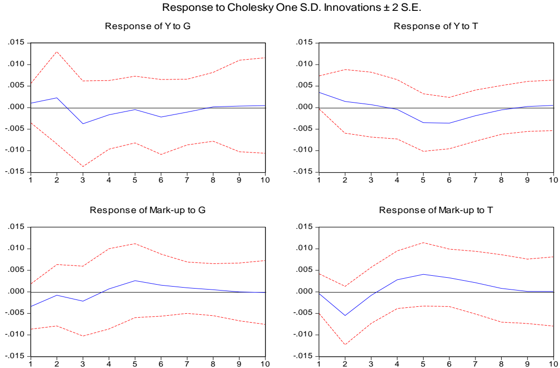
Figure 2: The impulse response functions: Denmark
