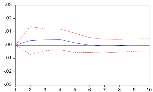
Response of PTF to T
