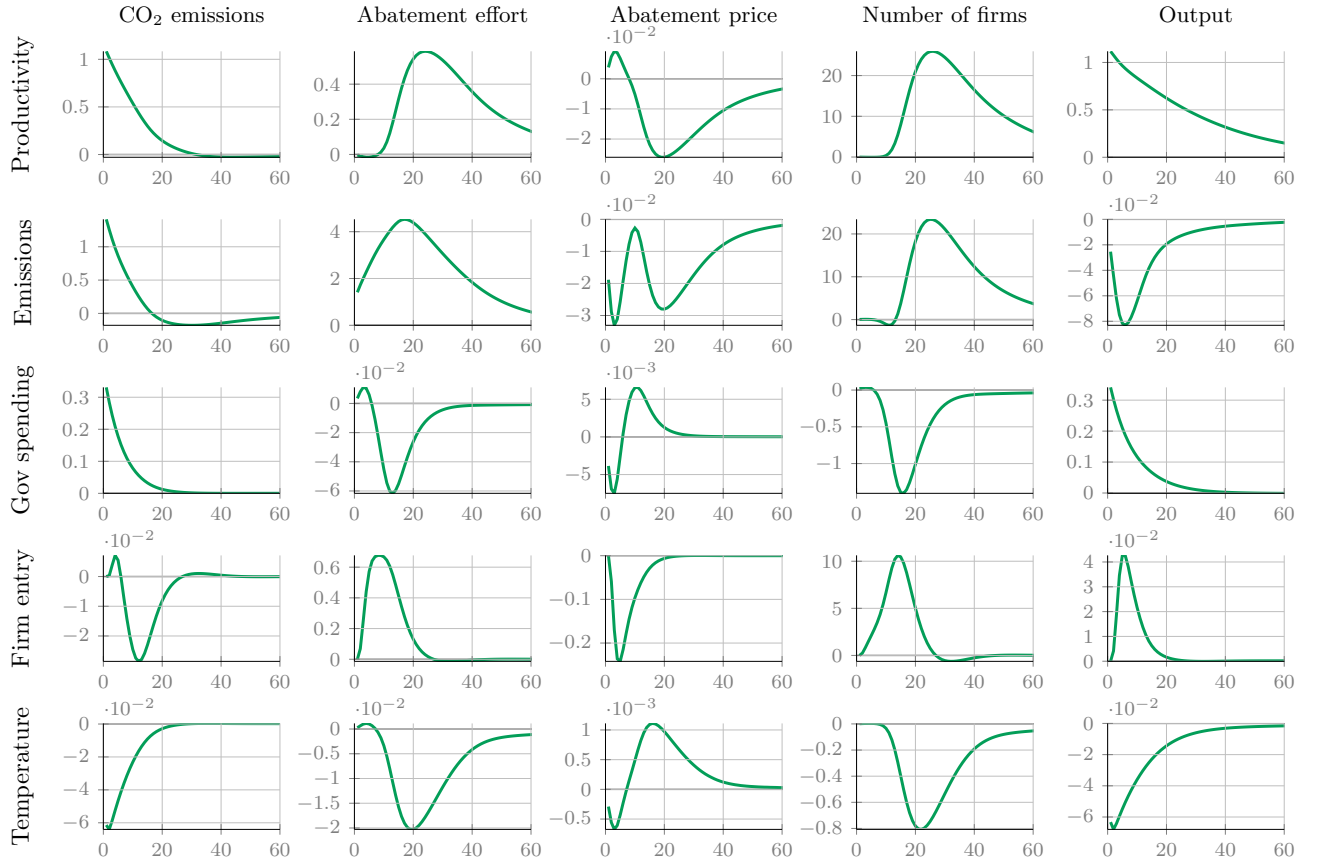
FIGURE 3. Generalized impulse response functions
