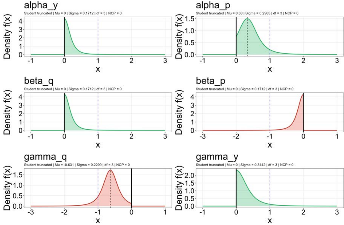
Figure A.1: Priors for the contemporaneous coefficients in \mathbf{A}
