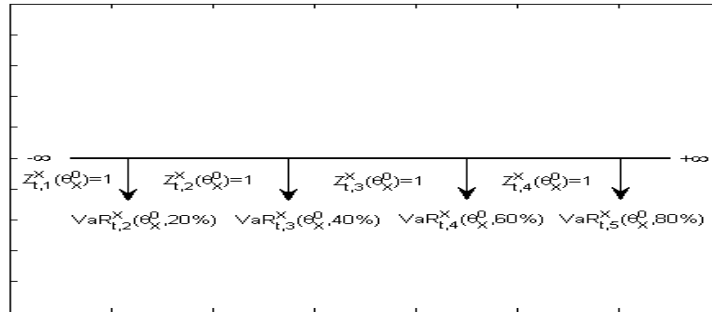
Figure 1: Distribution support of X and localization of VaRs and event variables
