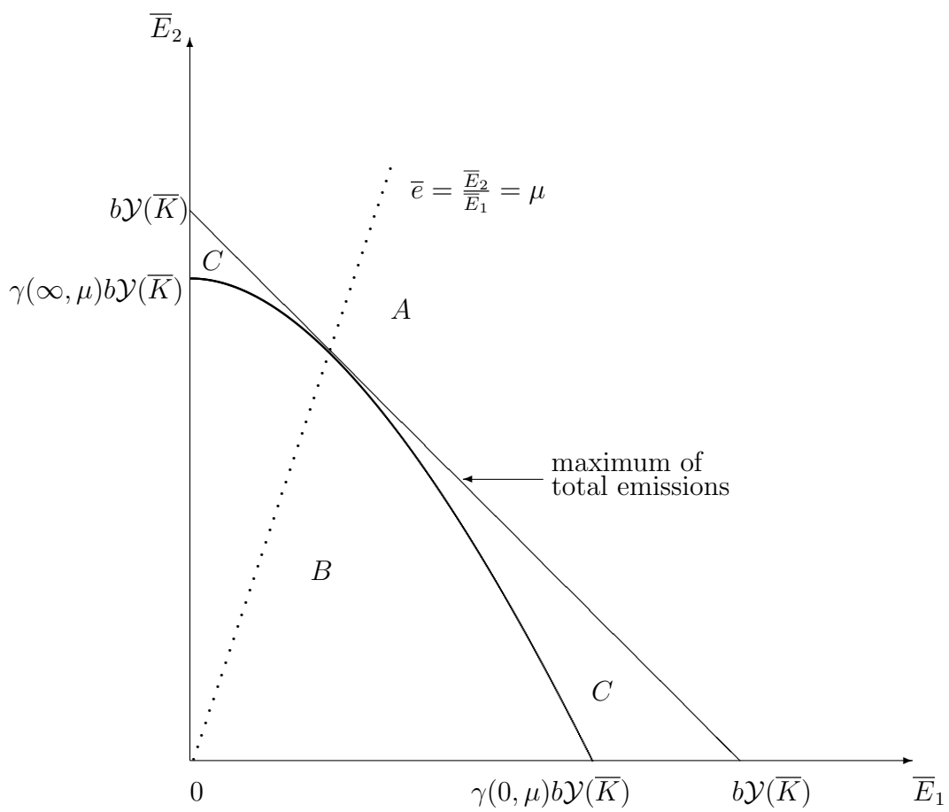
Figure 1: Regions corresponding to different types of equilibrium.
