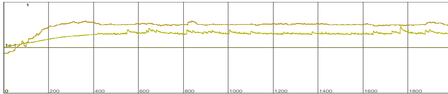
Figure 4: 10 \cdot \text{Mark-Up} (orange) and Price (yellow)
