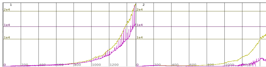
Figure 13: Output (yellow), final consumption (magenta)
