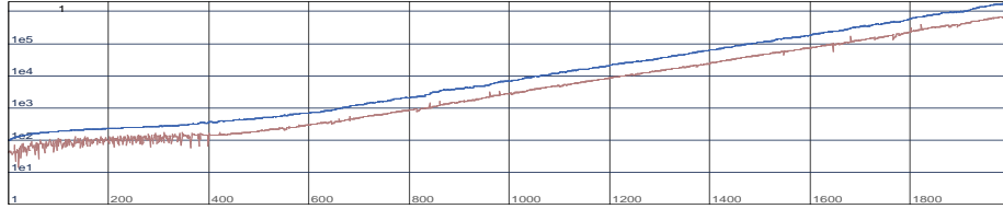
Figure 7: Output (blue) and Consumption (pink), log. scale
