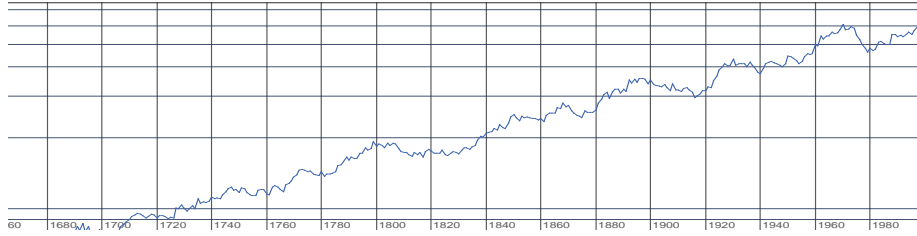
Figure 1: Output (rate of expectations change 0.2) , log. scale from 10^7 to 7.10^7
