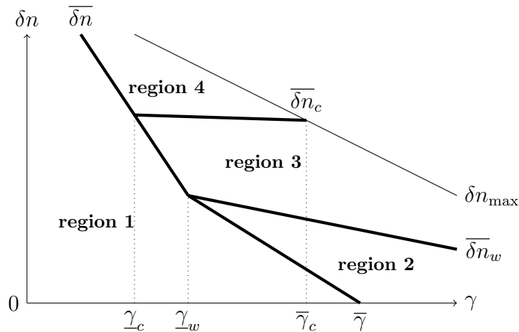
Figure 1: The four regions of Proposition 5
